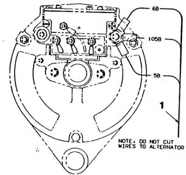
VIEW AP ALTERNATOR SCALE 1:1
