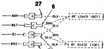
VIEW BG 27 RIGHT FRONT PROXY SWS NO SCALE
