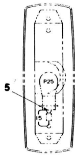
VIEW F LEFT TURN SIGNAL SCALE 1:1
