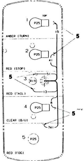
REAR VIEW H LEFT REAR COMBO LIGHT STOP, TURN, TAIL, FOG & BACK-UP SCALE 1:1
