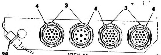
VIEW AA CARRIER HARNESS CONNECTORS SCALE 1:1
