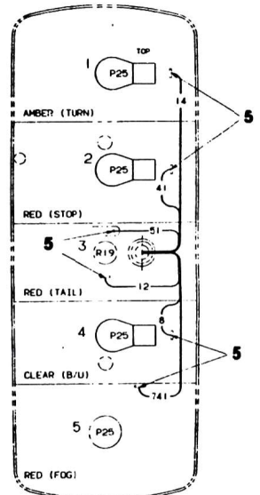
REAR VIEW C RIGHT REAR COMBO LIGHT STOP, TURN, TAIL, FOG & BACK-UP SCALE 1:1
