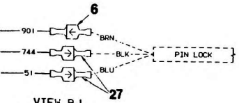
VIEW BJ PIN LOCK PROXY SW NO SCALE
