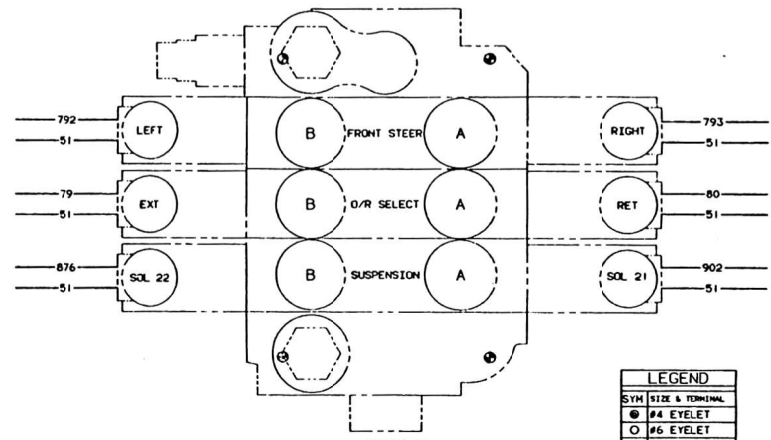
VIEW U FRONT STEER SOLS D/R SEL SOLS SUSPENSION SOLS SCALE 1:1
