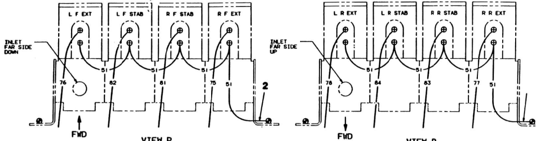
VIEW R REAR D/R SOLENOIDS BOTTOM VIEW SCALE 1:1
