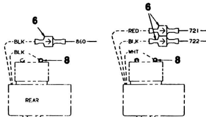
VIEW X INTER AXLE DIFF LOCK SOL SCALE 1:1
