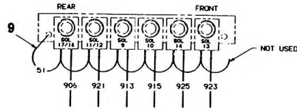
VIEW BB REAR AIR SUSP SOLS NO SCALE
