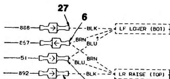
VIEW BH 27 LEFT FRONT PROXY SWS NO SCALE
