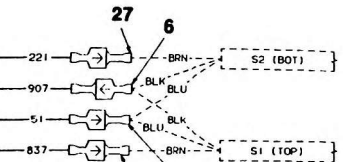
VIEW BK 27 REAR STEER LOCK PROXY SWS NO SCALE
