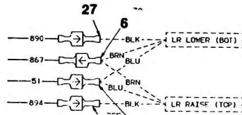
VIEW BE 27 LEFT REAR PROXY SWS NO SCALE
