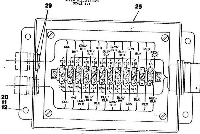
VIEW AN O/R JCT BOX SCALE 1:1
