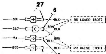
VIEW BD 27 RIGHT REAR PROXY SWS NO SCALE
