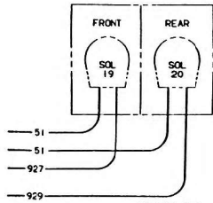
VIEW BA HYD SUSP LOWER SOLS NO SCALE
